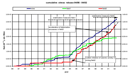
Figure 7: Cumulative stress release (BENIOFF-curve) of mining field1 (carnallite field), field2 (mixed salt field) and the entire mine
