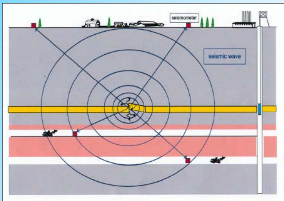
Principle of locating seismic events
