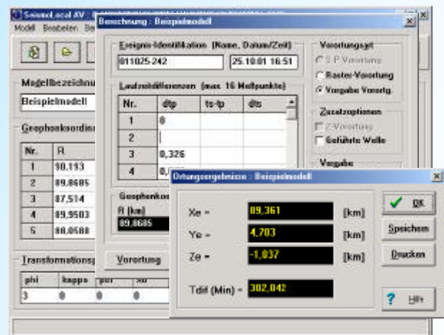
Tool SeismoLocal for locating local seismic events
