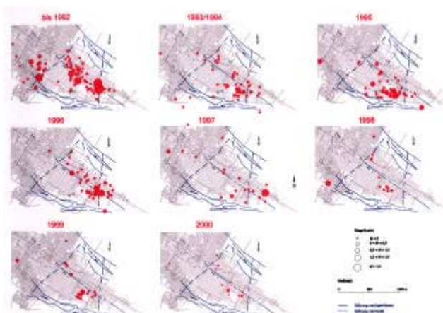
Figure 4: Development of the seismicity of a Carnallite mining field during (1991-1996) and after stabilization measures
