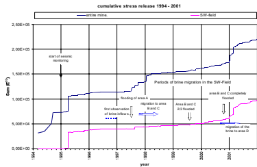
Figure 9: Cumulative stress release (BENIOFF-curve) of the flooded mining field and the entire mine
