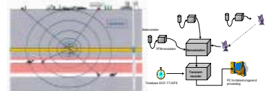
Figure 3: Scheme of a seismic monitoring network
